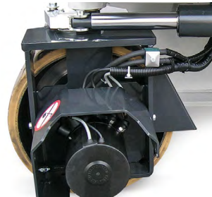
Standard negative electromagnetic parking brakes with electric disengagement
